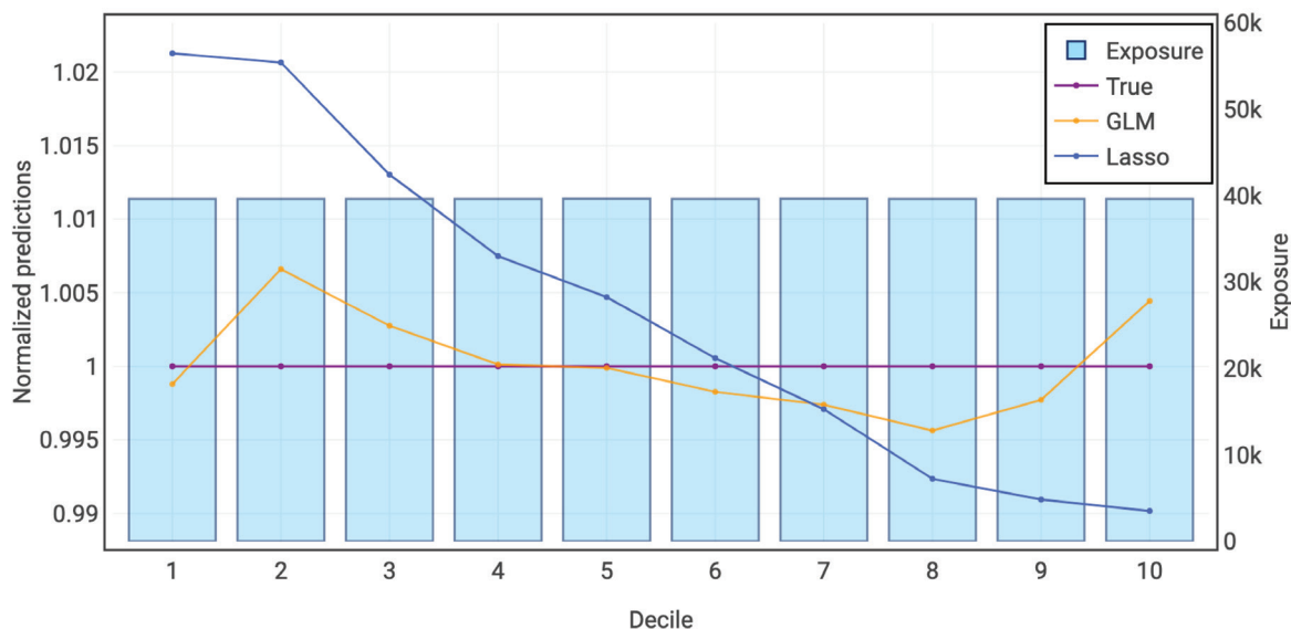
Figure 7.15. The GLM that Includes Insignificant Variables is Outperforming Our Penalized Regression Model by More Than 2% in the Lowest Decile
