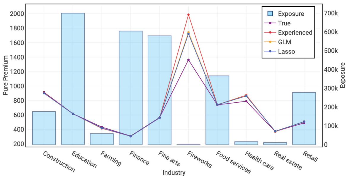
Figure 7.9. Neither Model is Able to Identify Situations Where the Experienced Pure Premium is Slightly Different Than the Experienced Pure Premium in Health Care and Fireworks
