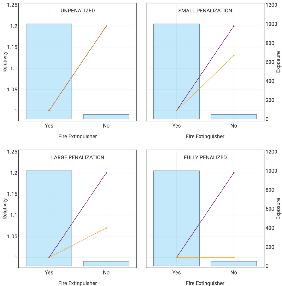
Figure 4.2. The experienced (purple) and the indicated relative (yellow) are shown across different values of penalization \lambda for the fire extinguisher variable. The experienced and indicated relativities completely overlap without penalization.
