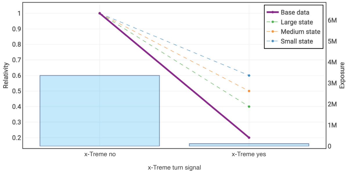
Figure 7.5. x-Treme turn signal has a very low relative that varies between data sets. We will use this example to show that lasso credibility can react—without overreacting—to strong signal in small segments.
