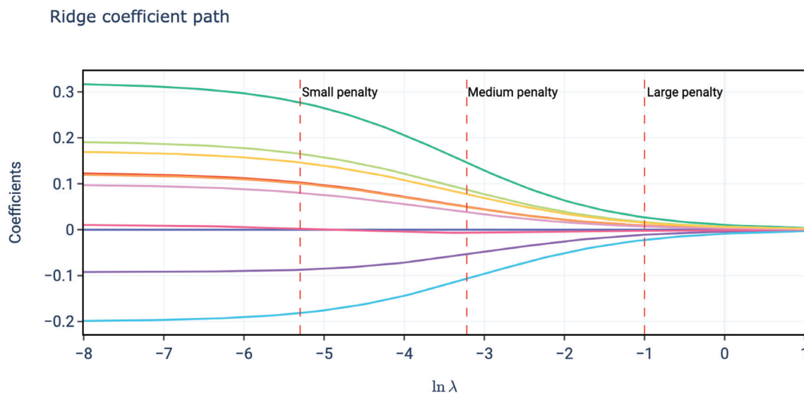
Figure 3.2. Coefficient path plot of Figure 3.1, obtained by computing solution for a wide range of penalty parameters. Dotted lines represent the values of \lambda penalty used to represent Figure 3.1. At very high values of the penalty (on the right), the coefficients are heavily shrunk and close to zero. Conversely, for very low values of the penalty, on the left, the coefficients are materially equal to the unpenalized GLM estimates.
