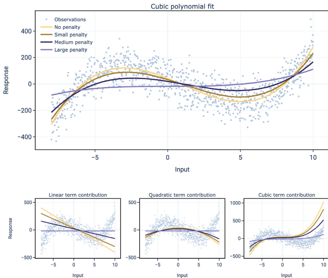
Figure 3.11. Lasso fit for various penalty values \lambda for a third-degree polynomial fit \beta_1x + \beta_2x^2 + \beta_3x^3 on a continuous variable. The top of the illustration represents the cumulated effect of the polynomial curve with different degrees of penalization, which results in an overall shrinkage of the curve. The bottom of the illustration provides the plot of the change of the individual polynomial function \beta_i x^i to the varying degrees of penalty.
