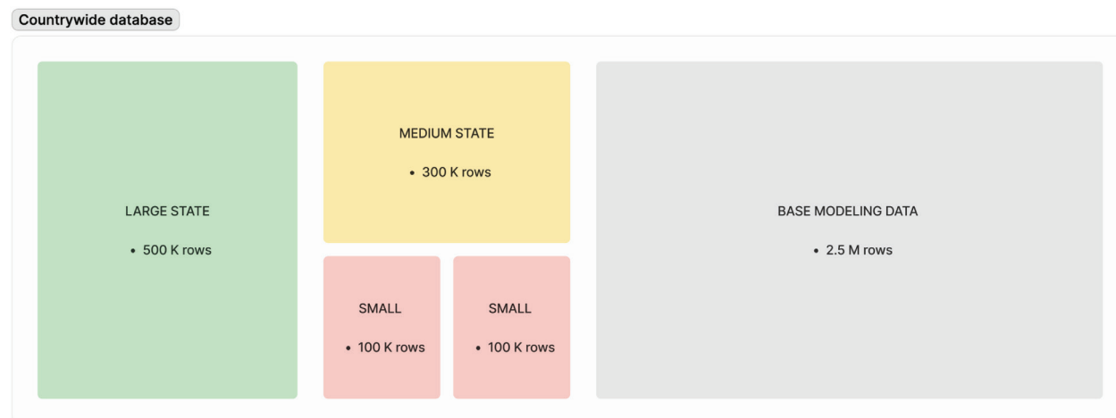
Figure 7.1. Visual representation of the various subsets in the simulated data. Risk characteristics are consistent within each subset but may (slightly) vary across states.
