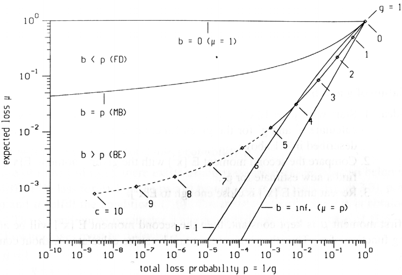
FIGURE 4.1: Range of parameters of the exposure curves G_{b,c}(x) . The expected value \mu is shown as a function of p = 1/g for special cases b = 0 , b = p , b = 1 and b = \infty . In addition, p and \mu are shown as a function of the curve parameter c for c = 0 \dots 10 . The dashed part of this curve has no empirical counterparts.
