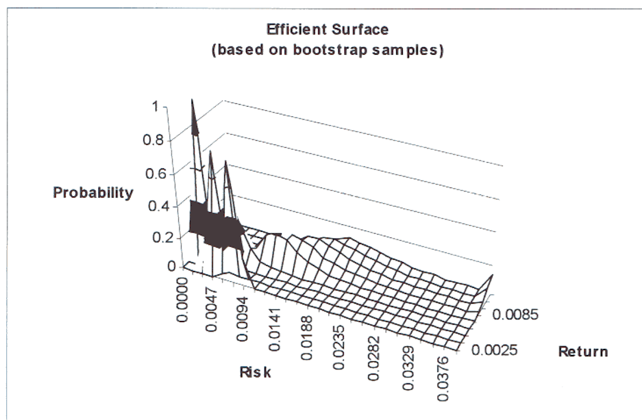
Figures 8 Views of EF Surface Created from Bootstrap Samples
