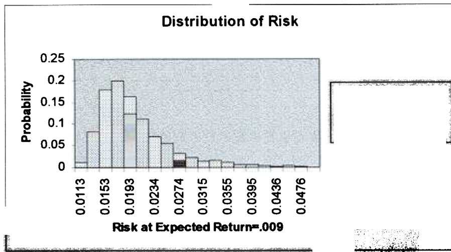
Figure 9 Dispersion of Risk Given a Return Level
