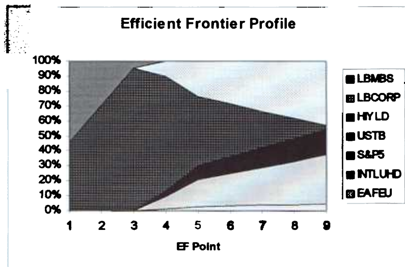
Figures 2b Portfolio Compositions for Different Efficient Frontiers
