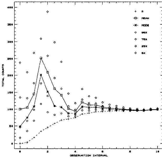
FIGURES 2a & 2b Predictive mean, mode, and fractiles versus t for Types Ic and IIc continuous data
